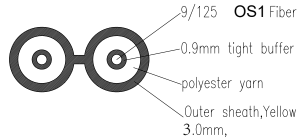
∅3.0mm cable section
